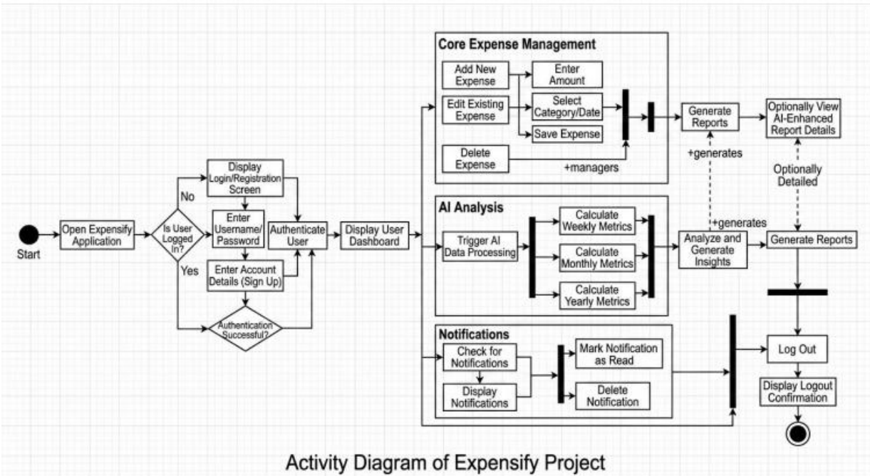
Figure 4.5: Activity Diagram
