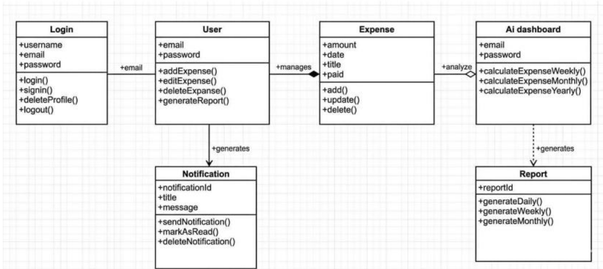
Class Diagram of Expansify
