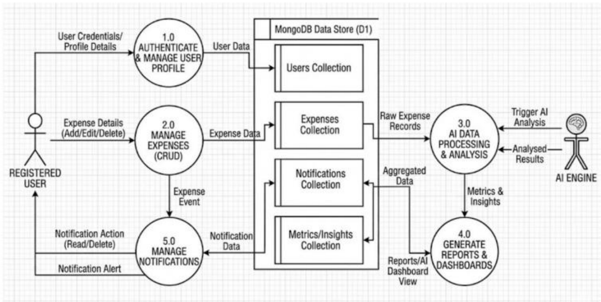
Figure 4.7: Data Flow Diagram
