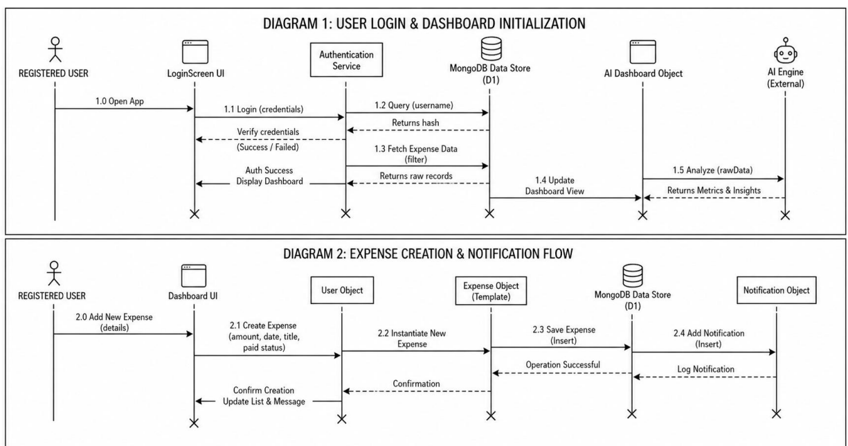
Figure 4.8: Sequence Diagram
