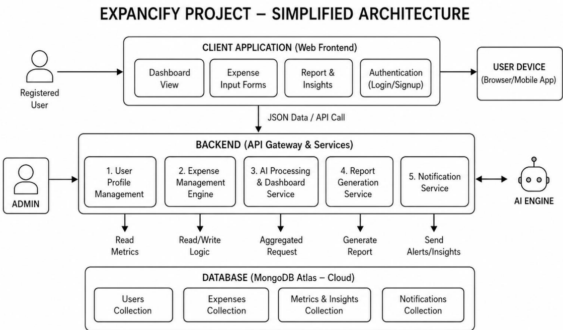
Figure 4.2: System Architecture Diagram
